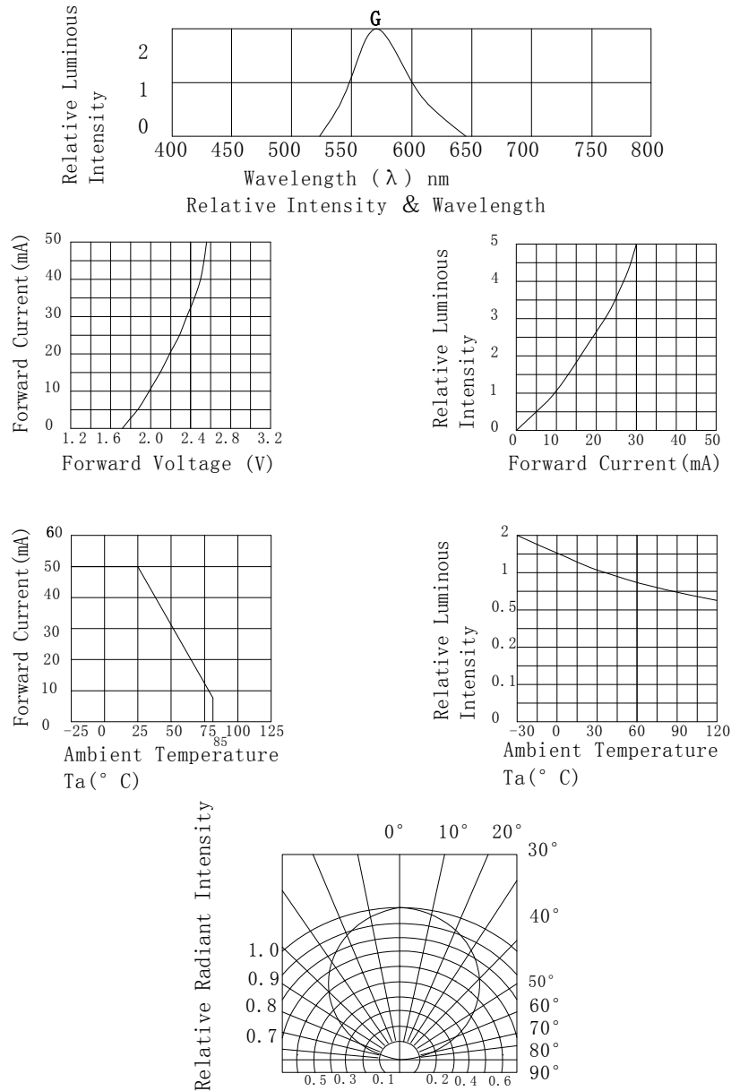
Fig.6 Radiation Diagram
