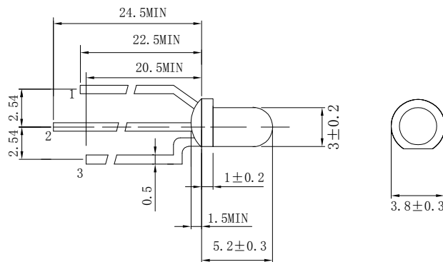
FDL-322HRG-ZW1-CA(Common Anode)
