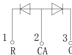
FDL-322HRG-ZW1-CA(Common Anode)
