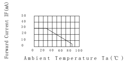
Forward Current Derating Curve
