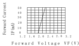
Forward Current vs. Forward Voltage
