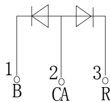
FDL-3522RB-ZWC1-CA (Common Cathode)
