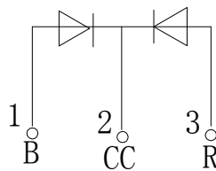
FDL-3522RB-ZWD1-CC (Common Cathode)
