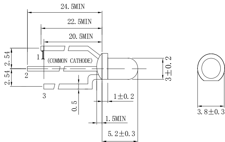
FDL-3522RB-ZWD1-CC (Common Cathode)
