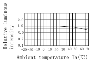
Relative Luminous Intensity vs. Ambient temperature
