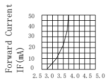
Forward Current vs. Forward Voltage
