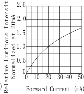
Fig.4 Relative Luminous Intensity VS. Forward Current
