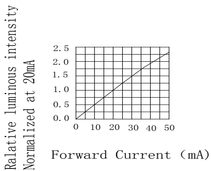
Forward luminous Intensity vs. Forward Current
