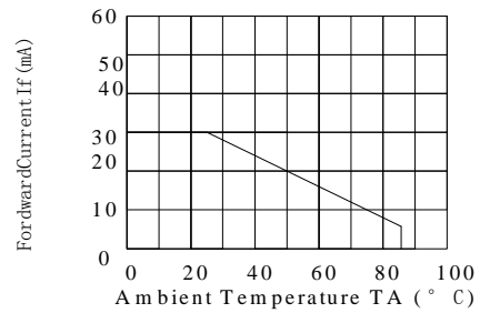
Fig.3 Forward Current Derating Curve
