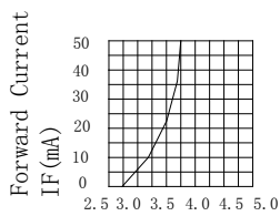
Forward Current vs. Forward Voltage
